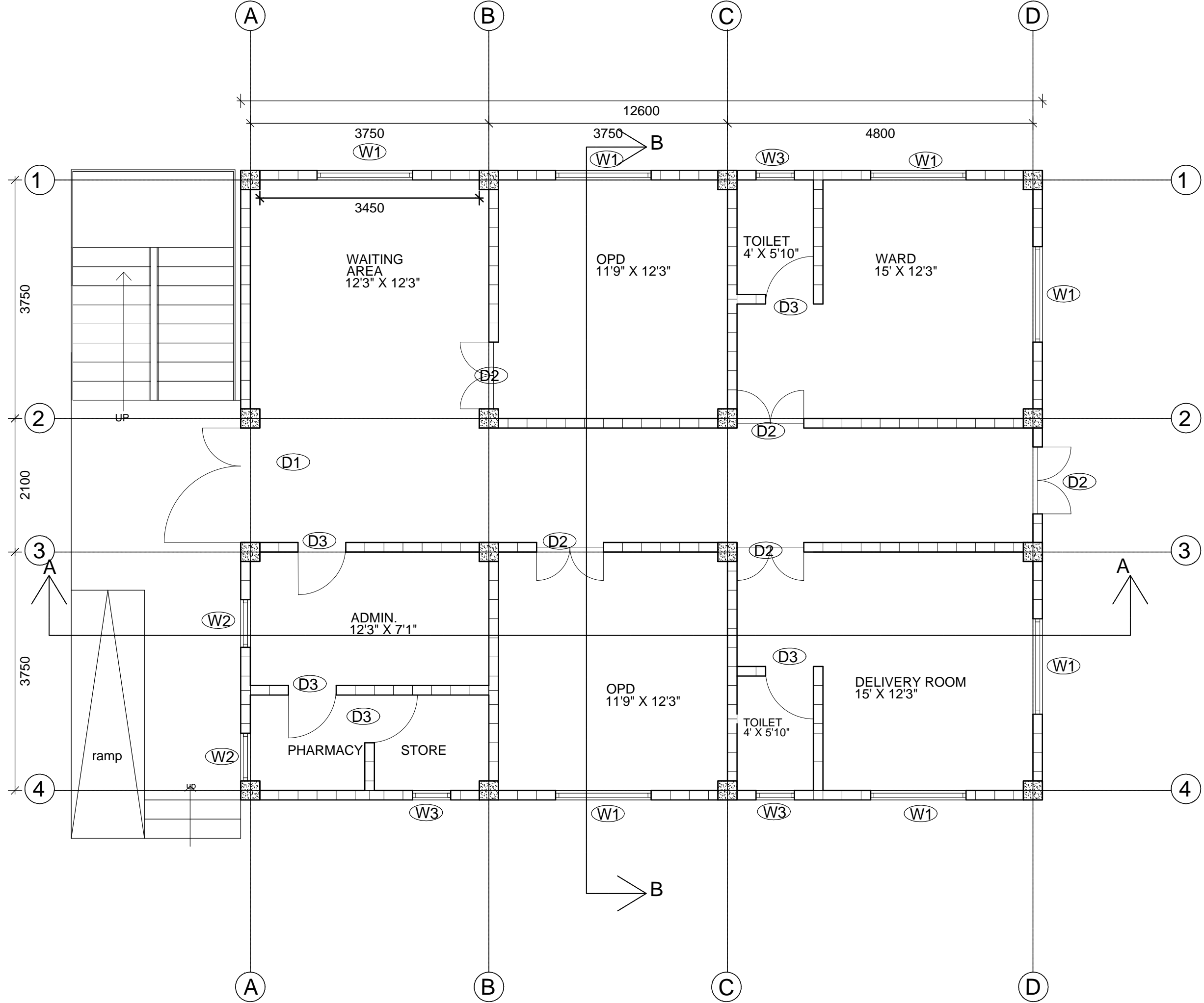
GROUND FLOOR PLAN HEALTH POST AT THOKARPA
